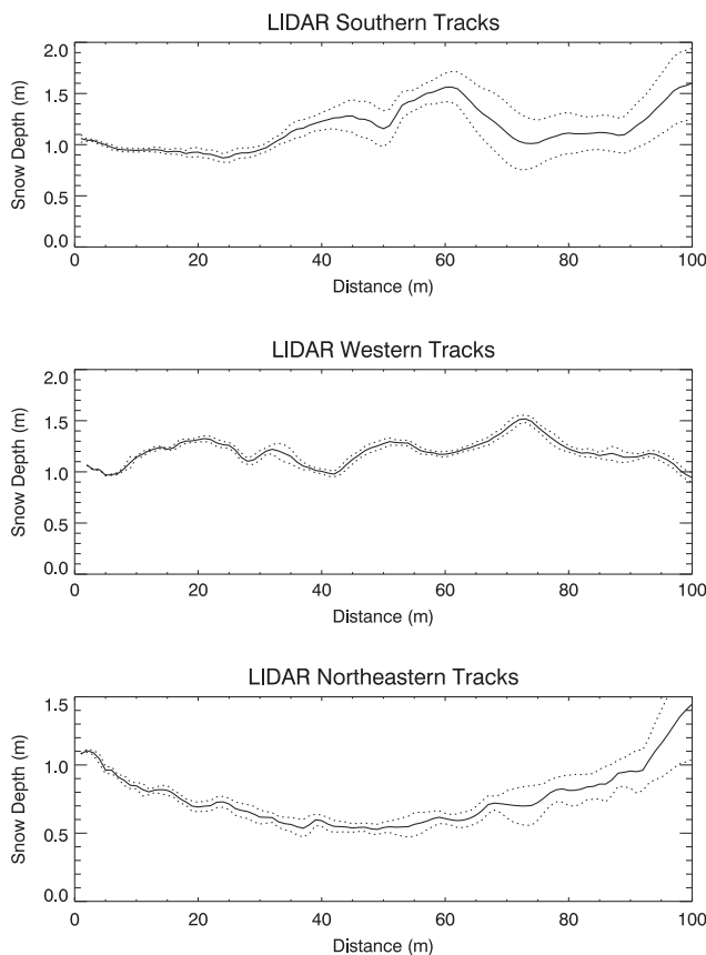
Figure 9. Snow depth profiles from LIDAR data for three GPS regions, southern tracks (top), western tracks (middle) and northeastern tracks (bottom); in all cases, the GPS is at 0 m on the x -axis. Mean (solid line) is plotted with one standard deviation above and below (dotted line)
